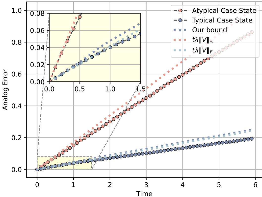
2D-lattice QIMF, long-time evolution with imperfections
